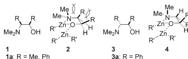
Figure 1. Chiral amino alcohols 1 and 3 , and their complexes 2 and 4 with organozinc species.
