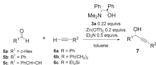
Scheme 1. Chiral amino alcohol 3a -mediated catalytic asymmetric alkynylation of 5 with 6 .
