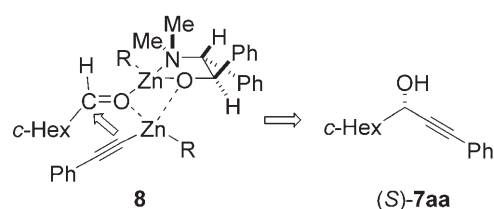
Figure 2. Model 8 predicting the stereochemistry of ( S )- 7 .
